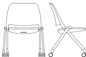
ZP21 LS 18" HD 15.5" HS 18" PS 17" PT 25"
