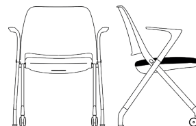
ZE33 LS 18.5" HD 15.5" HS 18.75" PS 17" LT 27.5"
