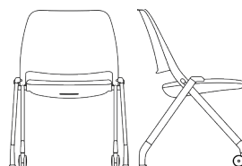
ZP23 LS 18" HD 15.5" HS 18" PS 17" PT 25"
