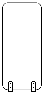
IWL2454 TW 24" TD 15" TH 54"
